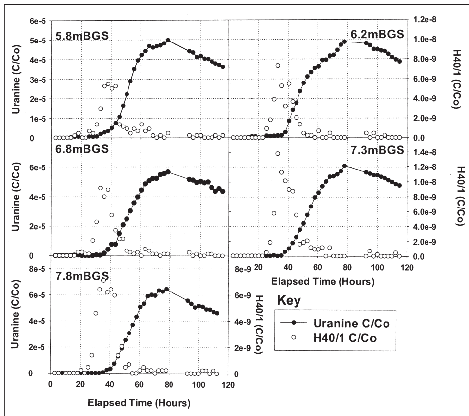
Fig. 4: Breakthrough curves for five different depths sampled using a multi-channel low-flow sampling system at K3-2, Kappelen Test Site, Switzerland. C/C_o – injectate concentration, m BGS – metres below ground surface.
