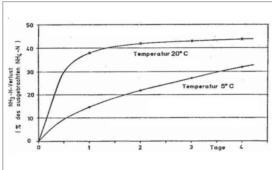
Fig. 2.1: Wirtschaftsdüngerenausbringung: Ammoniakverluste (%) temperatur- und zeitabhängig. NH 3 -N – Ammoniak, NH 4 N – Ammoniumstickstoff. Spreading of organic manure: Loss of ammoniac (%) due to temperature and duration until the beginning of tillage operations [days]. NH 3 -N – ammonia, NH 4 N – ammonium.
